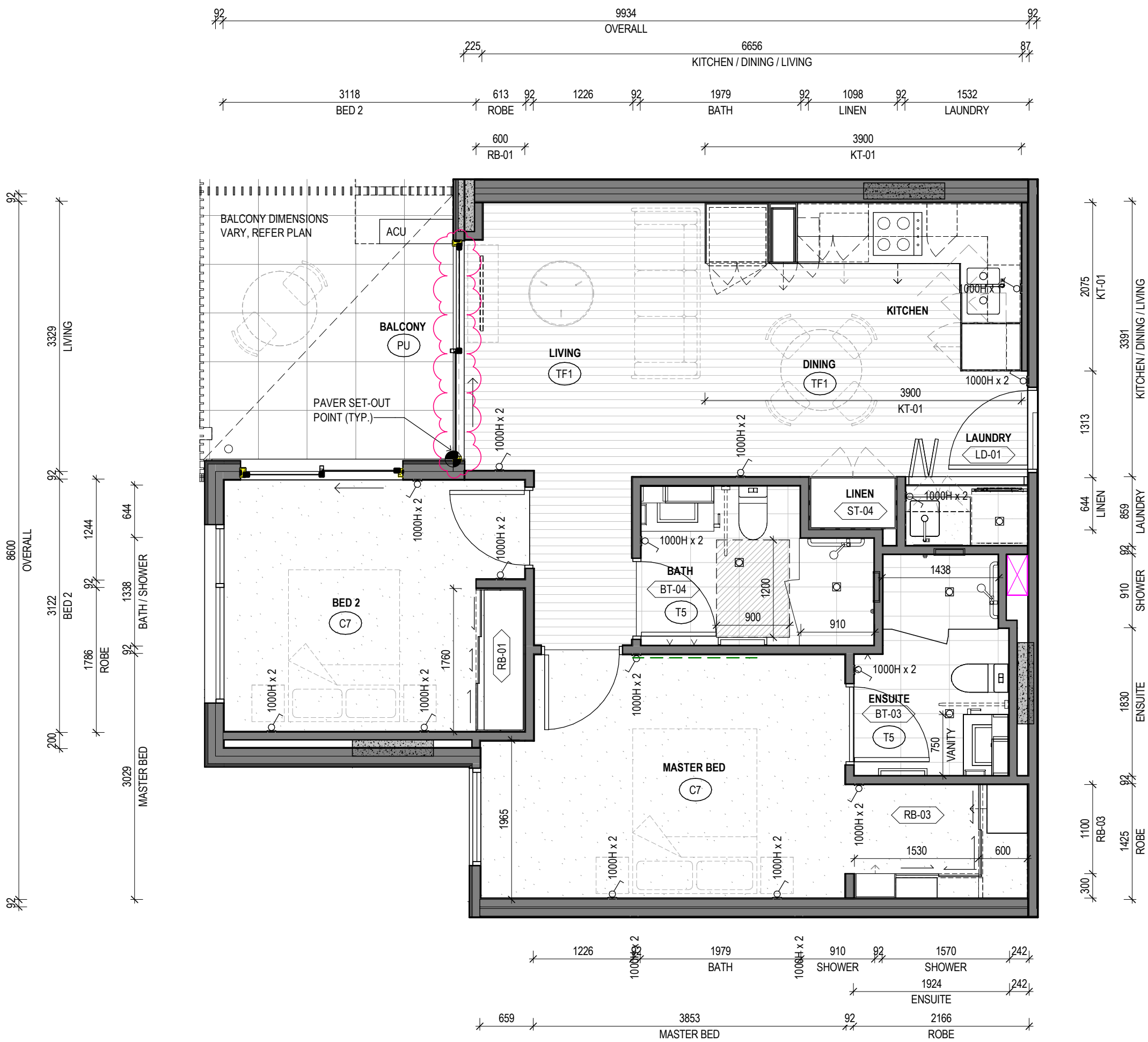
1 ILA Type 8 Scale 1: 50
